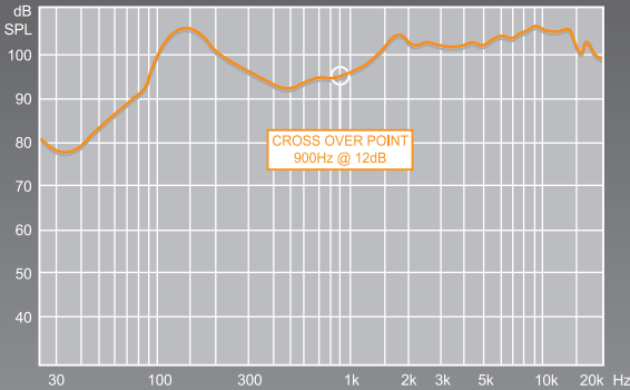
Freq Resp
